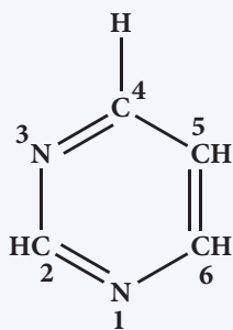
Pyrimidine
