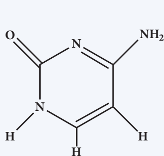
Cytosine (C)
